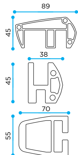
Profiel details
